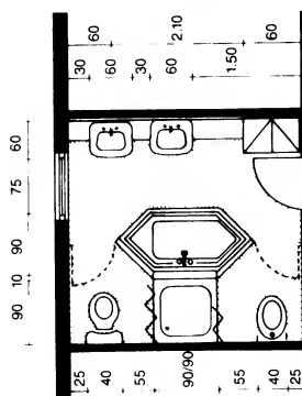
⑯ Spacious bathroom
